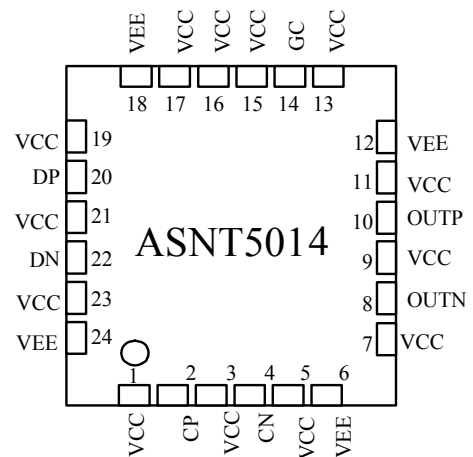
Package Pins
