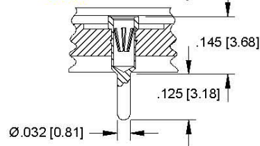
-295V Socket Assembly
