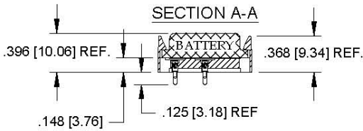
-280V Socket Assembly
