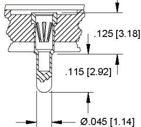
-280V Socket Assembly
