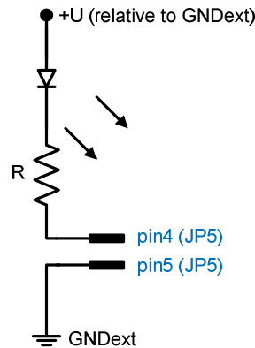
Fig. 13 Example of using an open-collector alarm output of JP5 to illuminate an external LED. The load R limits the current to max. 20 mA.
