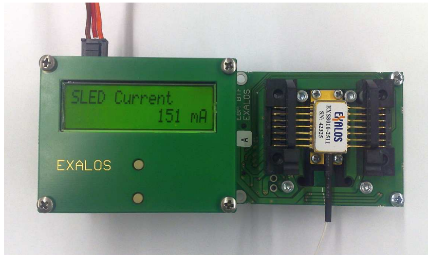
Fig. 4 Top view of an EBD5020 with an adapter board for 14-pin BTF modules
