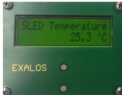
Fig. 9 Display-Board DIB5000 in display mode 3 (SLED temperature)
