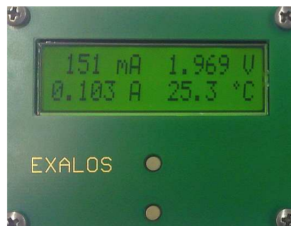
Fig. 11 Display-Board DIB5000 in display mode 0 (all four parameters)
