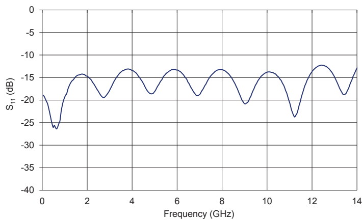
MX2000-LN-10 Typical S_{11} Curve
