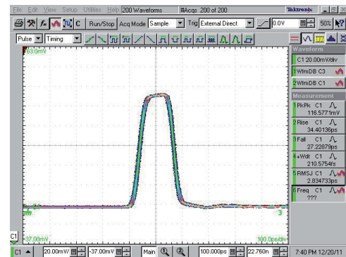
Output response
